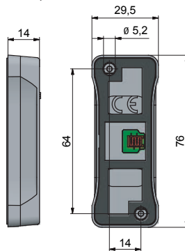
RFID reader L033-A03 with spacer
