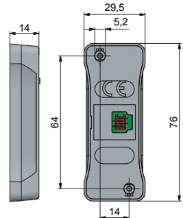
RFID reader L043-A02 with spacer
