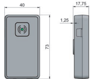
RFID reader L043-A01 (internal mounting)
